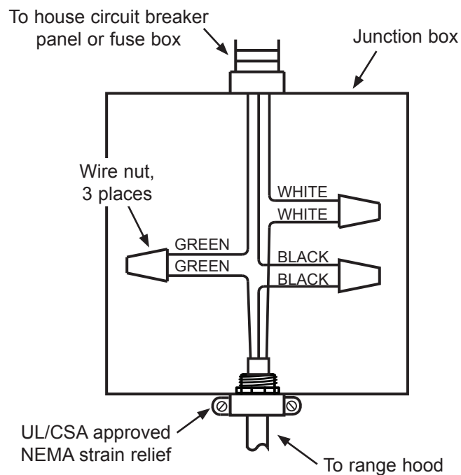
3 Wire Connection to Junction Box
