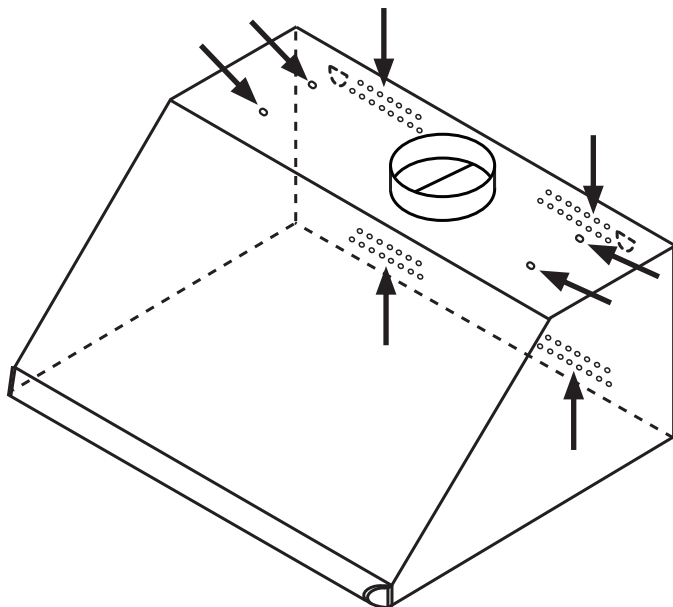
Mounting Hole Locations
