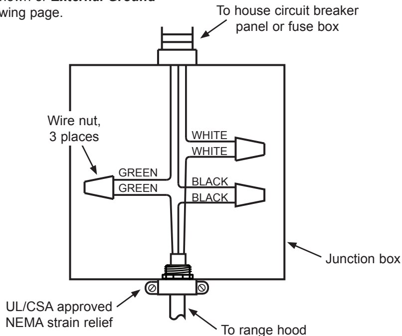
3 Wire Connection to Junction Box
