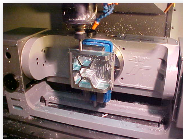
U.S. 5 Axis Machining Mill
