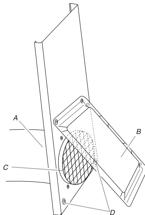
A. Window exhaust adapter D. Bolts inserted into unused holes in window slider kit B. Rain cover C. Outlet grille
