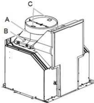
A. Air outlet B. M4*12 Screw C. Remove the tape from the flapper
