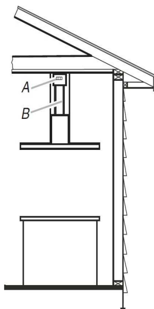
A. Chimney hole B. 6" (15.2 cm) round vent
