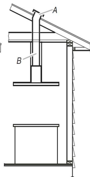
A. Roof cap B. 6" (15.2 cm) round vent
