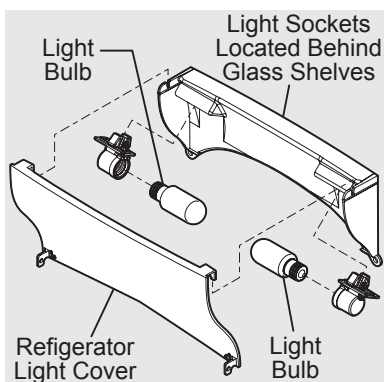
Refrigerator Light
