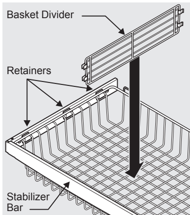
Basket Divider
