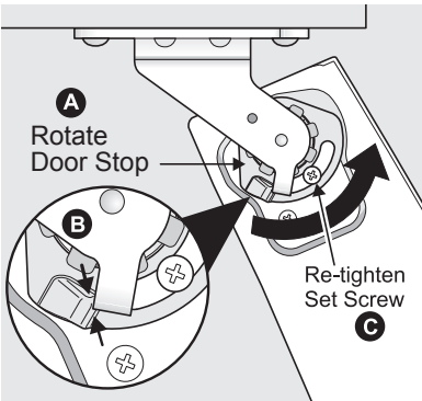
Retighten Screw
