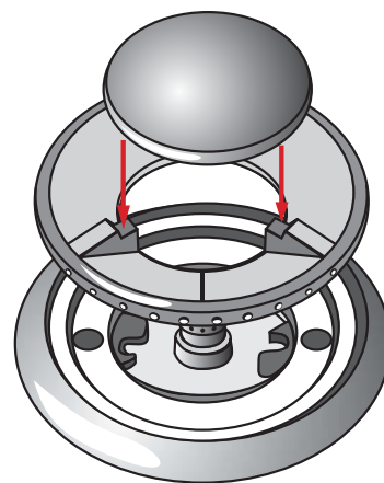
Figure 5 - Correct G5 Burner Cap Placement
