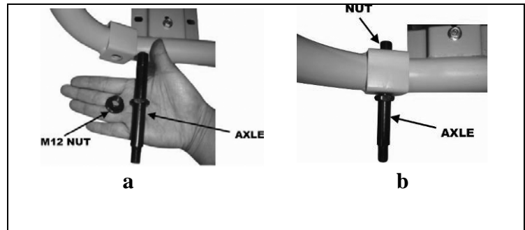
Figure 5- axle assembly
