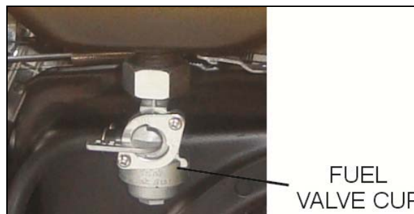
Figure 24- Removing the Fuel Filter Cup
