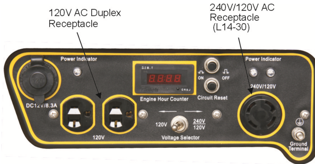
Figure 17- Receptacles available on the generator
