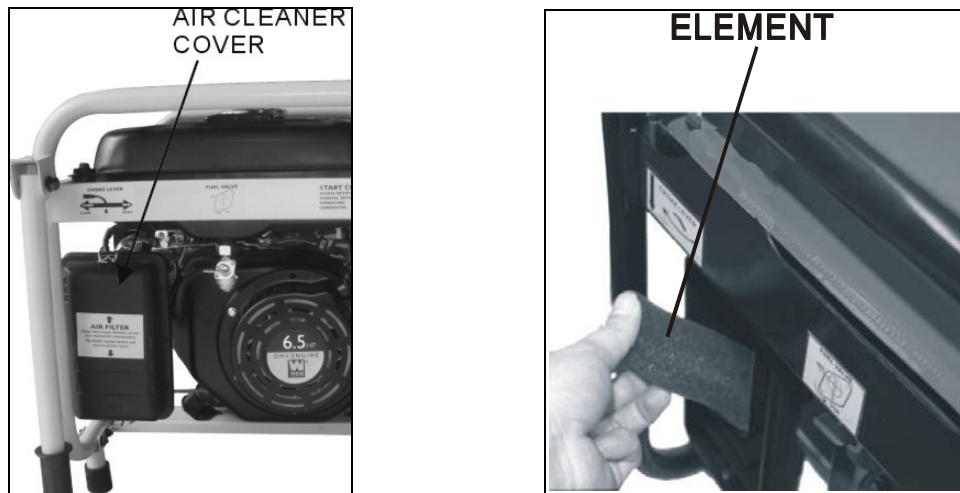
Figure 23- Removing the air cleaner casing.
