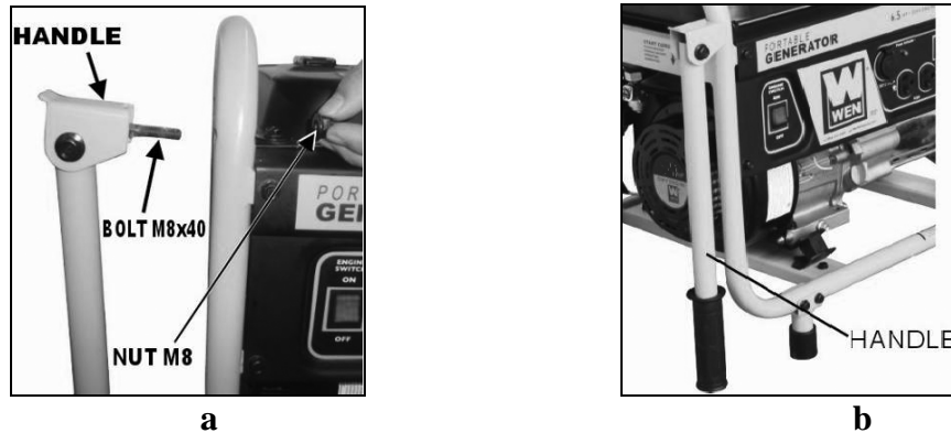
Figure 3- handle assembly
