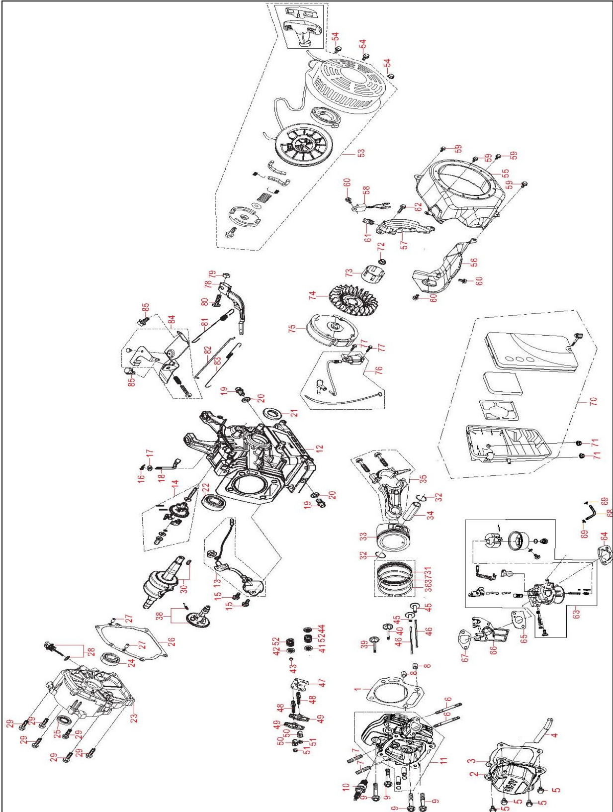
Engine exploded view
