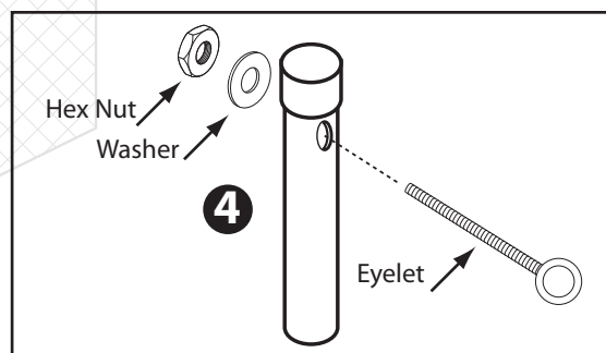
Connector Detail
