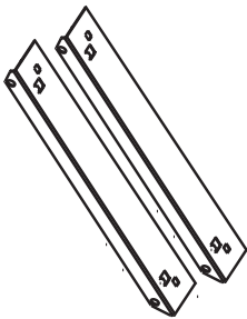
Long Upper Support Brackets (18-1/16 in.)
