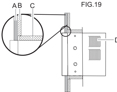
A. Plastered wall B. Inside wall C. Wood frame D. Louvers
