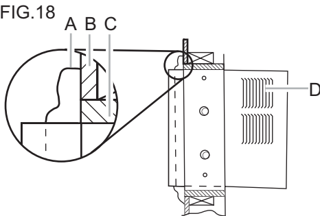
A. Molding B. Inside wall C. Wood frame D. Louvers
