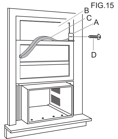
A. Window lock bracket B. Upper window glass C. Window sash seal D. #10X1/2" round-head screws
