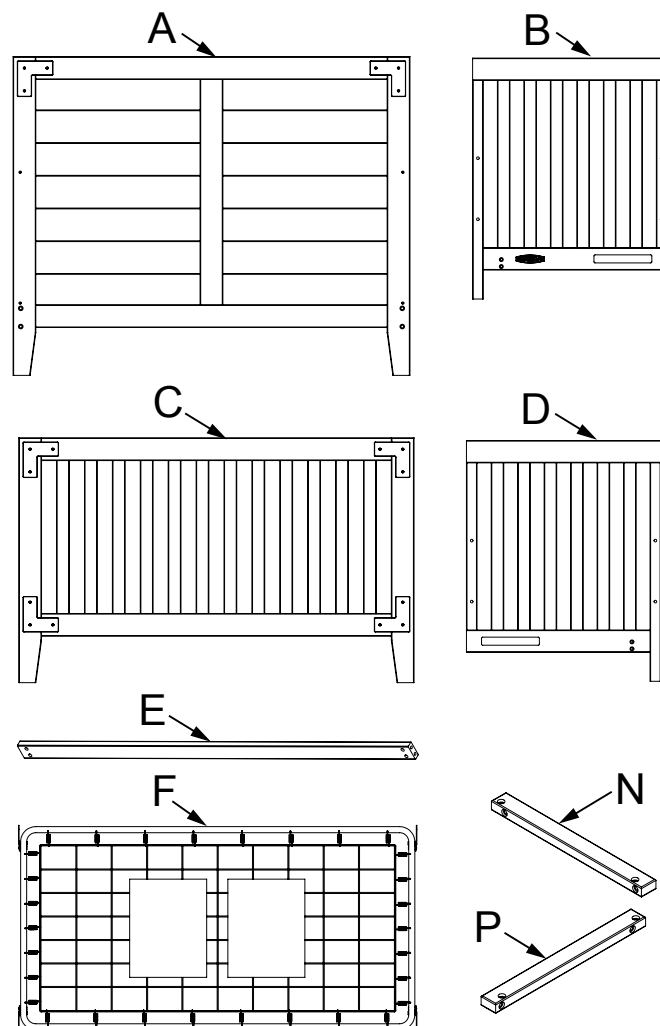
Crib Parts
