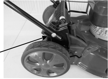
M8 Screw, Nut and washer
