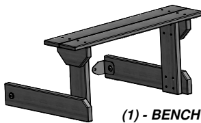
(1) - BENCH ASSEMBLY
