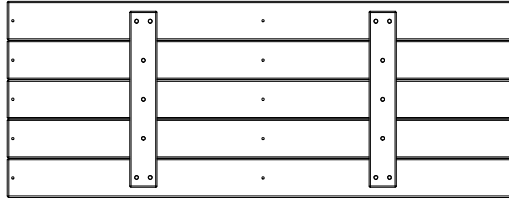
(2) FP1 - FLOOR PANEL - W103717 1 1/4"x17"x44 3/8" (32x432x1128)
