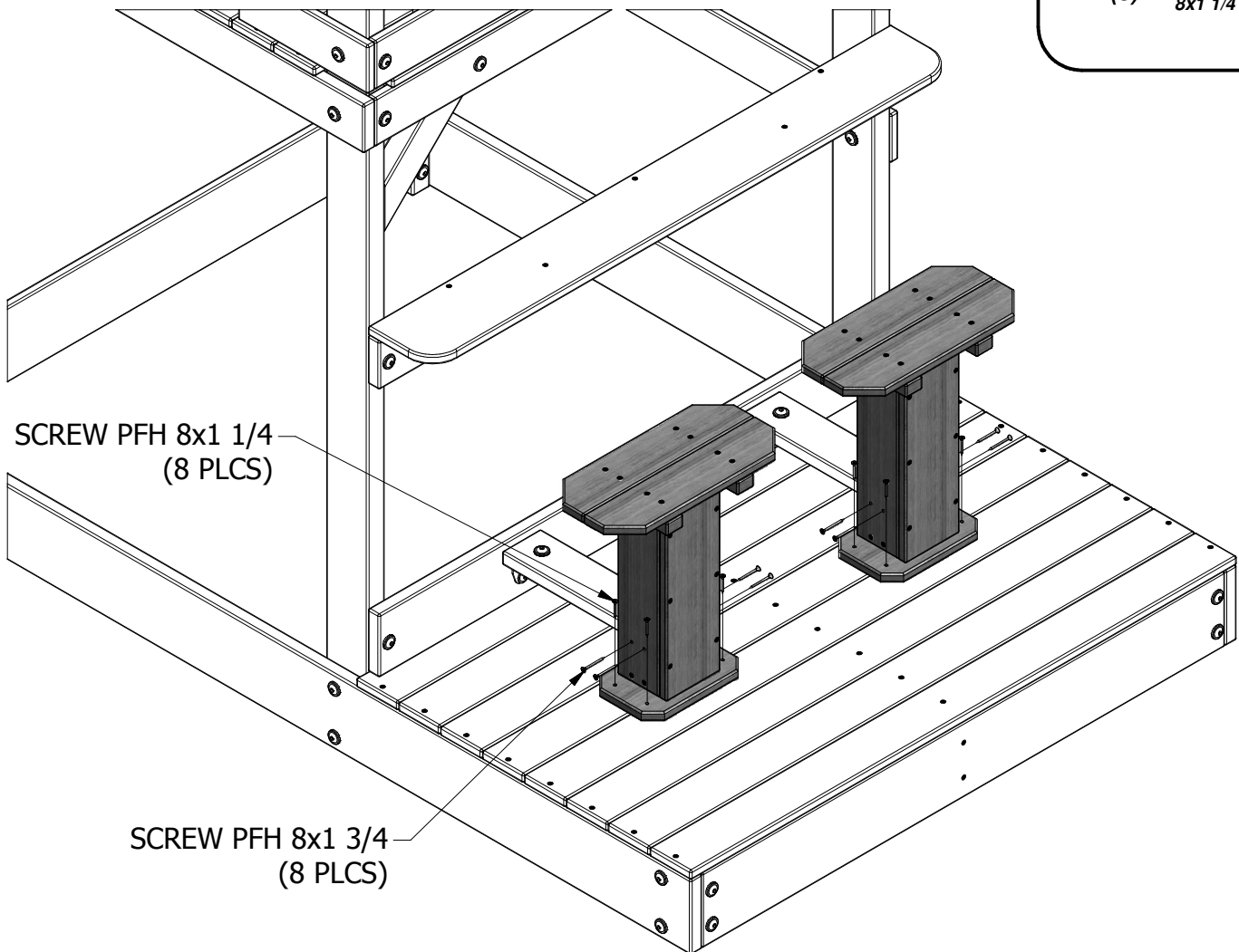
(8) SCREW PFH 8x1 1/4
