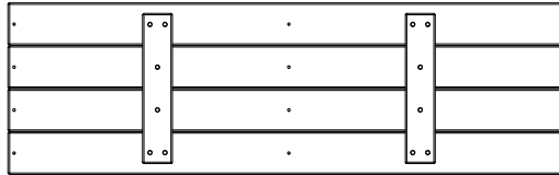
(2) FP2 - FLOOR PANEL - W103725 1 1/4"x13 5/8"x44 3/8" (32x346x1128)
