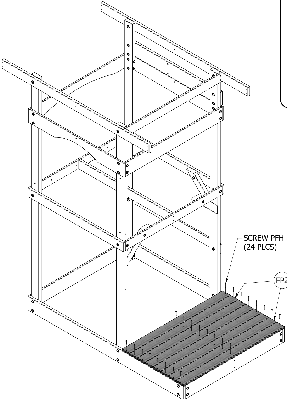
(24) SCREW PFH 8x1 3/4
