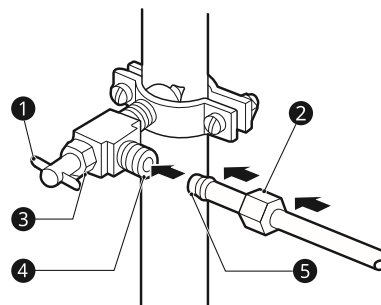
a Saddle-Type Shutoff Valve
