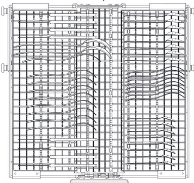
Third rack load pattern for 8 place settings.
